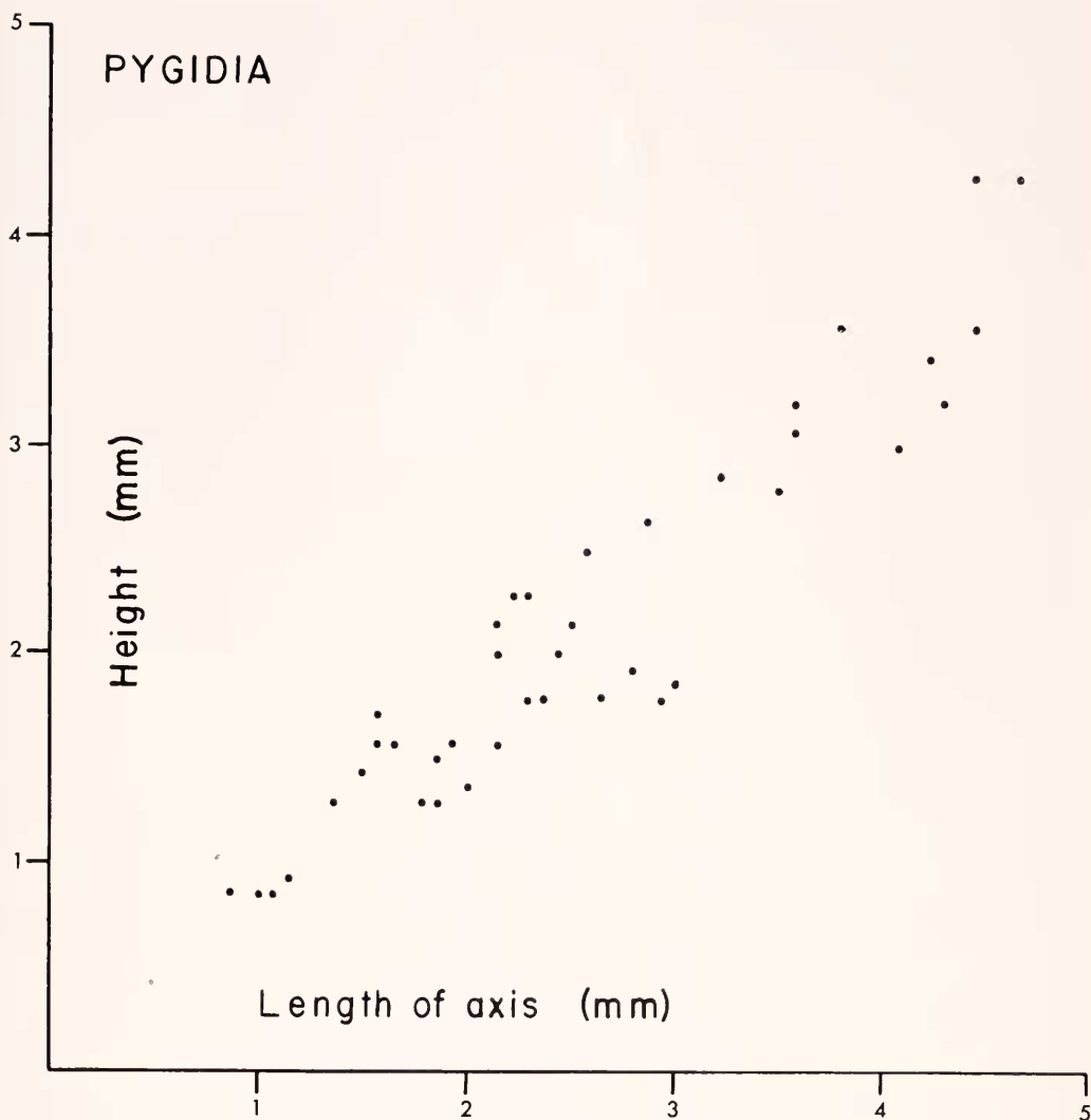
Figure 5. Proetus pluteus n. sp. Dimensions of 40 pygidia, length of axis is sagittal, height is maximum. Measured specimens the same as Figure 4.
